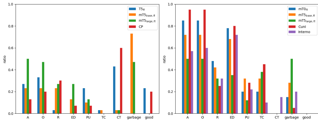
Figure 5: Error ratio per model. English (Left) and Russian (Right).
