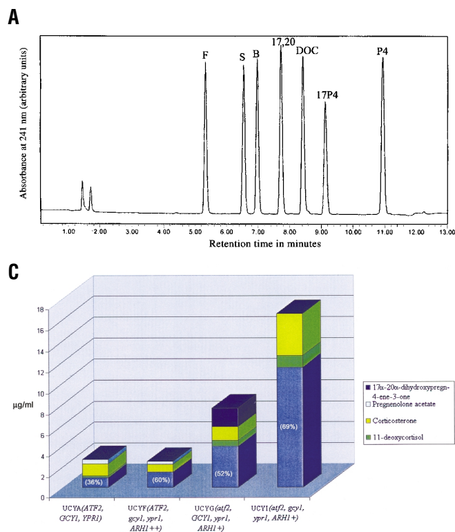
Figure 2. Steroid productivity of selected strains. (A) HPLC profile of a standard mix of purified steroids. (B) HPLC profile of a typical steroid extract from UCYH pCV29/pCC12. F, Hydrocortisone; B, corticosterone; S, 11-deoxycortisol; 17,20, 17 \alpha ,20 \alpha -dihydroxypregn-4-ene-3-one; DOC, deoxycorticosterone; 17P4, 17 \alpha -hydroxyprogesterone; P4, progesterone. (C) Steroid productivity ( \mu g/ml) of selected strains: UCYA ( ATF2 , GCY1 , YPR1 ); UCYF ( ATF2 , gcy1 , ypr1 , ARH1 ++ ); UCYG ( atf2 , GCY1 , ypr1 , ARH1 + ); UCYI ( atf2 , gcy1 , ypr1 , ARH1 + ), see Table 2 and Experimental Protocol. Concentration of the different produced steroids and percentage of hydrocortisone are indicated. Both parameters could be substantially improved by suitable disruptions of endogenous yeast activities and overexpression of Arh1p.
