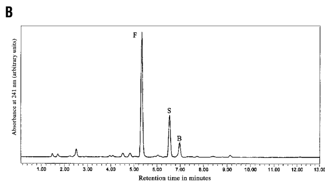
Figure 2. Steroid productivity of selected strains. (A) HPLC profile of a standard mix of purified steroids. (B) HPLC profile of a typical steroid extract from UCYH pCV29/pCC12. F, Hydrocortisone; B, corticosterone; S, 11-deoxycortisol; 17,20, 17 \alpha ,20 \alpha -dihydroxypregn-4-ene-3-one; DOC, deoxycorticosterone; 17P4, 17 \alpha -hydroxyprogesterone; P4, progesterone. (C) Steroid productivity ( \mu g/ml) of selected strains: UCYA ( ATF2 , GCY1 , YPR1 ); UCYF ( ATF2 , gcy1 , ypr1 , ARH1 ++ ); UCYG ( atf2 , GCY1 , ypr1 , ARH1 + ); UCYI ( atf2 , gcy1 , ypr1 , ARH1 + ), see Table 2 and Experimental Protocol. Concentration of the different produced steroids and percentage of hydrocortisone are indicated. Both parameters could be substantially improved by suitable disruptions of endogenous yeast activities and overexpression of Arh1p.
