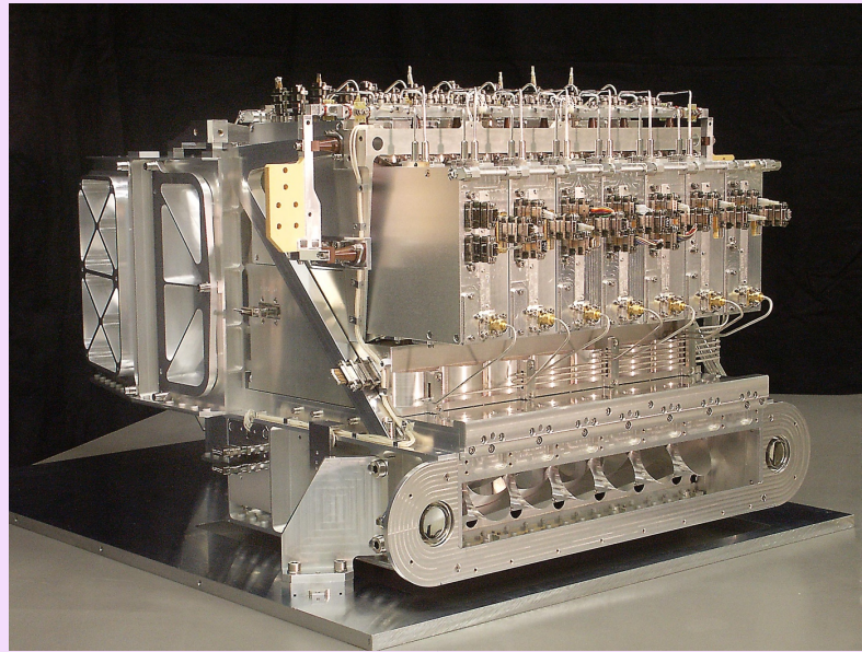
The HIFI Focal Plane Unit. This unit is located in the cryostat of the Herschel Space Observatory. Inside this unit are 14 superconducting heterodyne detectors that operated at 1.8 K in space.
