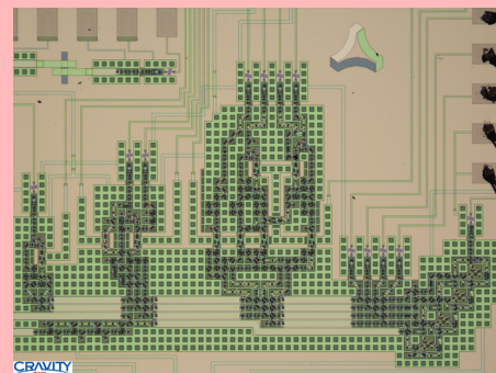
Arithmetic and logic units based on artificial neurons (XOR, Full adder, Multiplier) - 2019. Copyright: TOBB ETU
