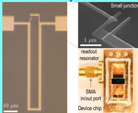
Fluxonium qubit 16
