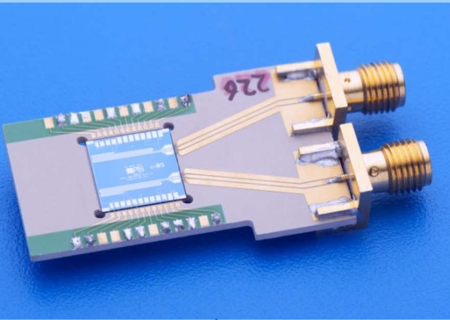
Single chip of the Josephson Arbitrary Waveform Synthesizer (JAWS) mounted in the sample holder. The JAWS is based on pulse-driven Josephson junctions. The 10 mm x 10 mm chip contains two series arrays of 12,000 Josephson junctions each [2018].
