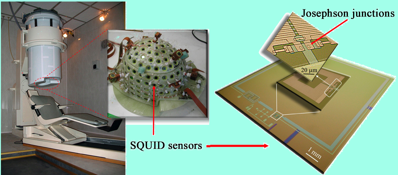
Left: Multi-channel MEG system with 165 sensors operating in a neurological clinic (Hermitage in Naples, Italy) 12 , the SQUID sensors are arranged in a helmet configuration to adapt to the anatomy of the skull. Right: SQUID magnetometer showing a field sensitivity of 1 fT/Hz 1/2 . The outer square loop transduces the field into magnetic flux in the SQUID with its depicted Josephson junctions.
