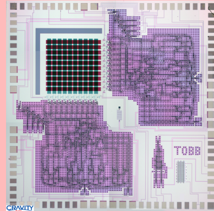
10x10 detector read-out and address encoder circuit-2017. Copyright: TOBB ETU
