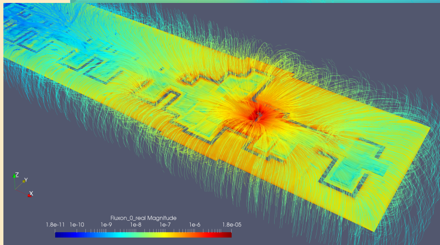
Extraction of magnetic flux lines of superconducting digital circuits. Copyright: Stellenbosch University and SunMagnetics, South Africa - 2023.
