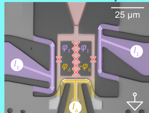
Cat-state qubit 17
