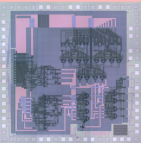
4-bit, pipelined Arithmetic-Logic Unit (ALU) - 2016. Copyright: TOBB ETU
