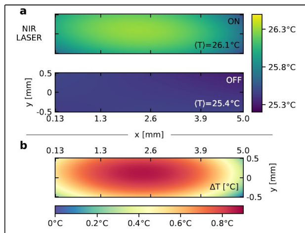
Fig.1: Map of the local temperature while illuminating the colloidal glass with the NIR laser. The laser enters the cell from the left-side of the maps (a): Local temperature during the NIR 'ON' and 'OFF' status, respectively. (b): Local change of T , calculated as the difference of the maps shown in panel (a). Figure adapted from [1].
