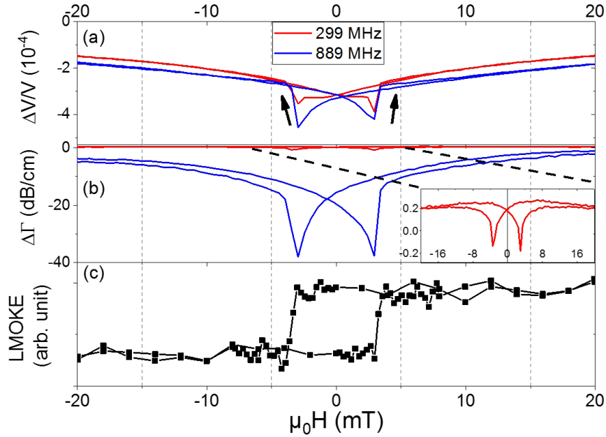
Figure 2: SAW-FMR experiment at T=130^\circ\text{C} , with the field applied along the SAW wavevector for f=299 and 889 MHz. SAW phase velocity (a) and amplitude (b) variations are shown versus applied field. The inset in (b) is a zoom on the 299 MHz curve. (c) Longitudinal Kerr cycle obtained by averaging a microscopy image of the FeRh mesa taken in front of the exciting IDT.
