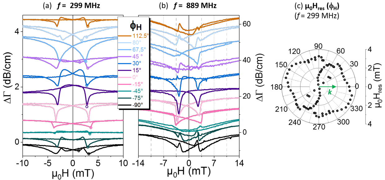
Figure 4: SAW-FMR at selected field angles (see the animations in the SI for the other angles) for (a) f=299 MHz and (b) f=889 MHz. (c) The resonance field H_{\text{res}} for f=299 MHz (open circle symbols in panel (a)) is shown as a function of the field angle \phi_H . \phi_H is counted with respect to the SAW wavevector direction (shown with the green arrow).
