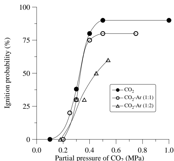
Figure 2 Ignition probability of spherical Mg particles (50-63 μm) in different CO 2 - Ar mixtures versus partial pressure of CO 2
