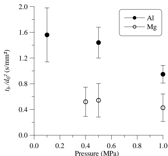
Figure 5 Effect of pressure on the inverse burning rate of Mg and Al particles in CO 2 ( t_b is the burning time, d_o is the initial size)
