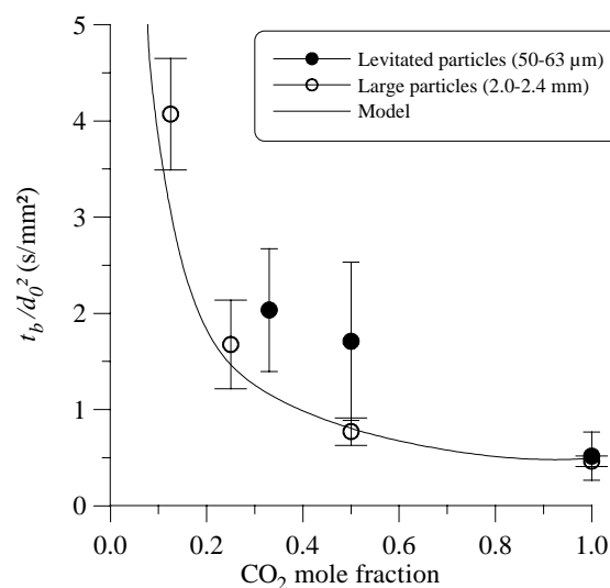
Figure 6 Comparison of measured burning times of levitated Mg particles in CO 2 and CO 2 /Ar mixtures with data for large particles [4] and with predictions by model [5]
