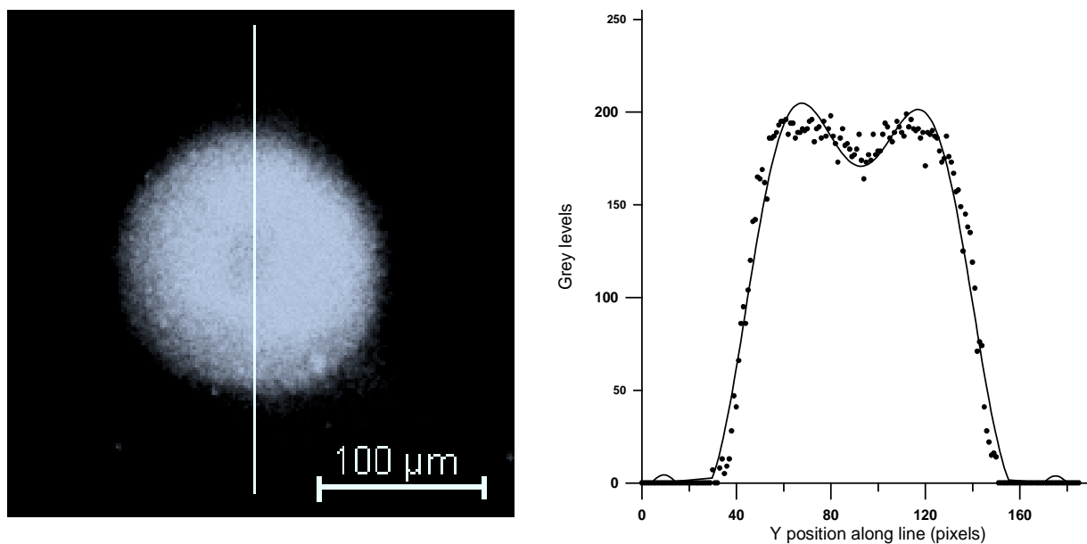
Figure 3 Image of a Mg particle ( \sim 60 \mu\text{m} ) burning in \text{CO}_2 and brightness of the image along the vertical line
