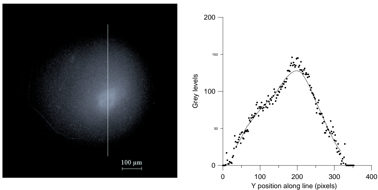
Figure 4 Image of an Al particle ( \sim 60 \mu\text{m} ) burning in \text{CO}_2 and brightness of the image along the vertical line
