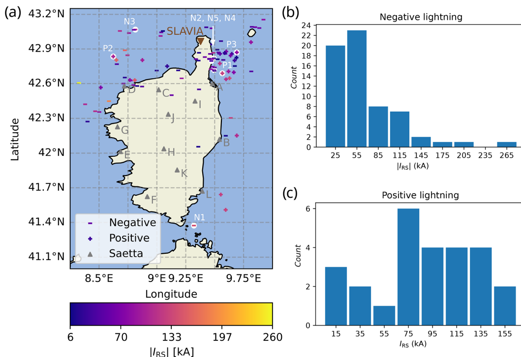
Figure 1. (a) Map of all first return strokes (RSs) used in this study, as located by METEORAGE. The -CG strokes are marked with “–”, whereas +CG strokes are marked with “+”. The colour corresponds to the absolute value of the first RS peak current ( I_{RS} ) for each flash. The SAETTA stations are labelled using grey triangles and their corresponding letter identifiers, while the SLAVIA sensor is marked using a brown upside-down triangle. The cartographic outline denotes the island of Corsica and the northern part of Sardinia. Panel (b) presents a histogram of the absolute value of the first RS peak current ( |I_{RS}| ) for all 66 -CG flashes. Panel (c) presents a histogram of I_{RS} for all 26 +CG flashes.
