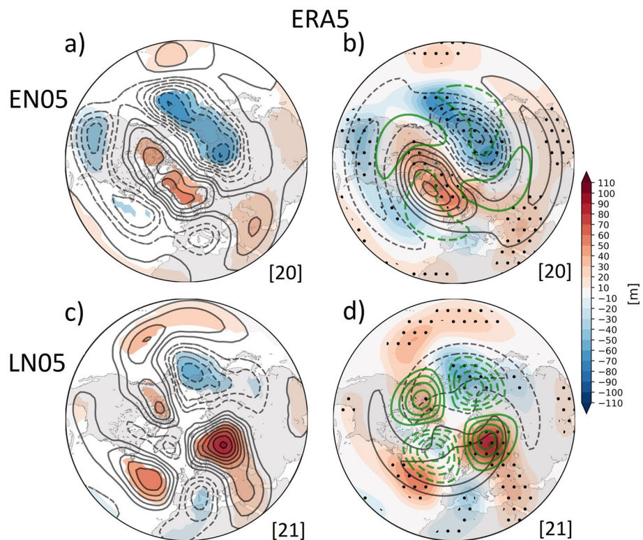
Figure 7. Anomalies of geopotential height at 500 hPa over the [-10, 0] -day period before SSWs in ERA5 for EN05 (top) and LN05 (bottom). (Left) same as in Figures 5e and 5i, but for EN05 (LN05). (Right), WN1 (black contours) and WN2 (green contours) components superimposed over the anomalies (shading). Note that contours in the left column correspond to the shading in the right column. Statistically significant areas at 95% confidence level according to a 1000-trial Monte Carlo test are shaded (dotted) in left (right) column.
