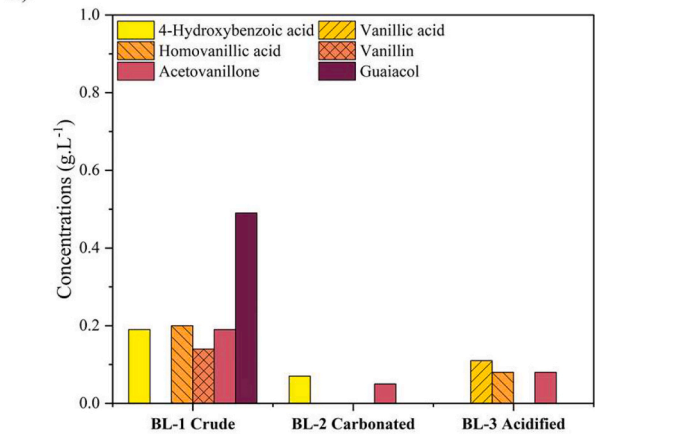
Fig. 7. Main aliphatic compounds (A) and phenolic compounds (B) identified and quantified in black liquors. Concentrations correspond to concentration values before dilution for HPLC analysis.
