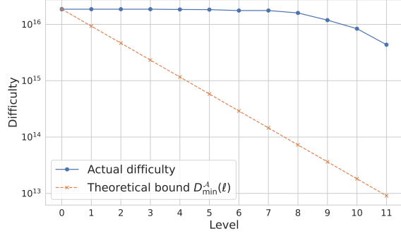
Figure 6: Comparison between the theoretical accumulated quantity of difficulty D_{\min}^A(l) and the one accumulated in the last K blocks of level l \geq 0 of the Bitcoin blockchain on October 11, 2024. Setting: K = 208 , \chi = 4032 , and k = 323 .
