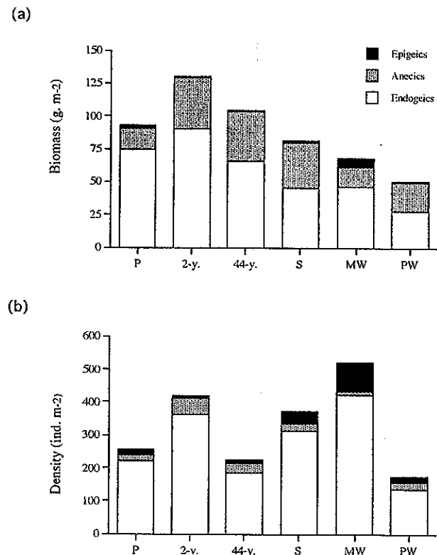
Figure 3. - Mean annual fresh biomass (a) and density (b) of earthworms in the six plots (P=pasture; 2-y.=2-year-old fallow; 44-y.=44-year-old fallow; S=scrub; MW=maple wood; PW=pine wood).
