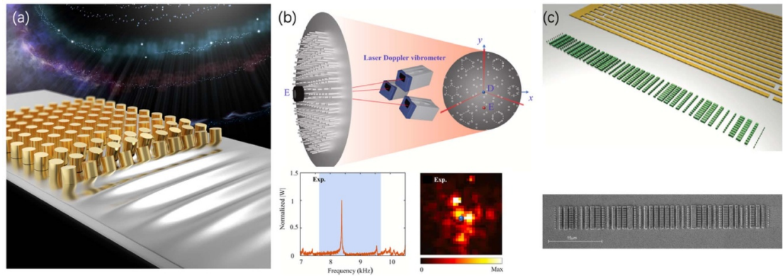
Figure 23. (a) Illustration of phononic crystals/acoustic metamaterials consisting of periodic pillars deposited on top of a plate which interact with Lamb waves. (b) Geometric structure of topological vortex mode for antisymmetric Lamb wave with Jackiw–Rossi binding mechanism. The lower panel shows experimentally measured response peak and out-of-plane displacement field of the topological vortex mode. Reproduced with permission from [208]. CC BY-NC 4.0 . (c) Illustration of SAW metasurfaces marked as green (upper panel) and fabricated sample (lower panel). Reproduced from [209]. CC BY 4.0 .
