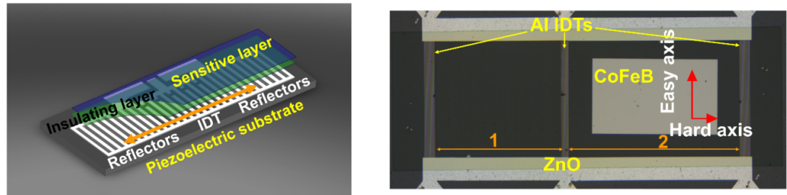
Figure 26. MSAW sensors. (a) Schematic view of a resonator configuration, with an insulating layer and a full film magnetoelastic layer. The SAW propagation direction is indicated in orange, (b) top view of a sample in delay line configuration with a CoFeB magnetoelastic layer between IDTs (path 2) and temperature compensation (path 1). Reproduced from [241]. CC BY 4.0.
