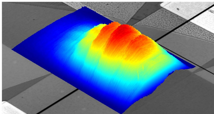
Figure 27. SAW wavefield measured in-situ at high temperature operation. Partial view of the amplitude distribution (shown in colour) of a CTGS-based 433 MHz resonator at 450 °C with local degradation of the electrode metallisation at the IDT-reflector transition.
