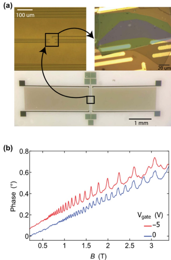
Figure 19. Observation of quantum transport in graphene using a surface acoustic wave resonator. (a) Optical microscope image of the device showing a view of the full SAW cavity in the lower image, an enlarged view of the of the centre of the cavity with the detail of the prepatterned gold electrodes without the graphene sample in the upper left image and a false-colour image showing the graphene device in detail in the upper right image. The monolayer graphene is coloured in light purple, and the graphite top gate is coloured in light green. (b) The change in the cavity phase at the fixed resonant frequency of the SAW resonator, as a function of magnetic field, at two different gate voltages, and at 1.7 K. The quantum oscillations are clearly visible above 0.6 T. The data have been offset for clarity. Reprinted (figure) with permission from [23], Copyright (2023) by the American Physical Society.
