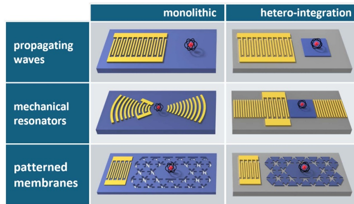
Figure 9. Possible implementations for dynamic modulation of QDs using acoustic phonon fields. These include dynamic modulation by a propagating SAW (top row), by the mechanical mode of a Bragg type resonator (centre row) and the modes of (suspended) phononic crystal resonators (bottom row). All these implementations can be done monolithically on the host substrate of the QDs (left column) or in hetero-integrated devices where QD membranes (blue) are transferred onto a different substrate (grey) (right column).
