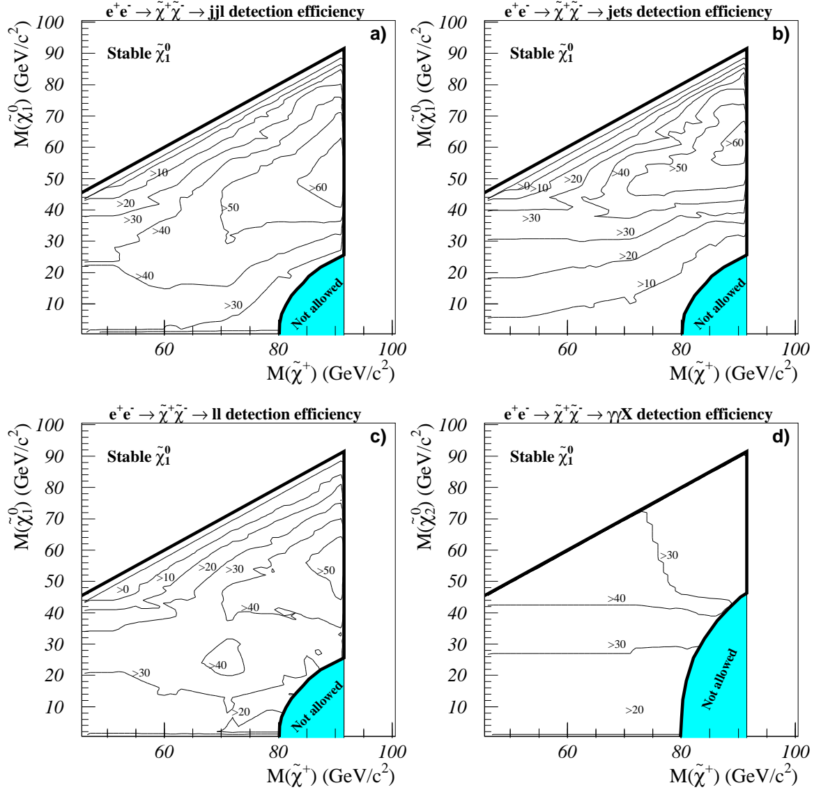
Figure 2: Chargino pair production detection efficiencies (%) for the 4 topologies a) jj\ell\ell , b) \text{jets} , c) \ell\ell and d) \gamma\gamma X , at 183 GeV in the (M_{\tilde{\chi}^\pm}, M_{\tilde{\chi}^0}) plane. A stable neutralino is assumed.
