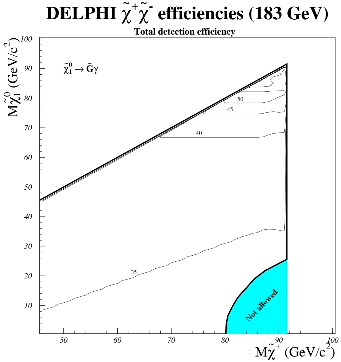
Figure 8: Chargino pair production detection efficiency (%) at 183 GeV in the (M_{\tilde{\chi}^\pm}, M_{\tilde{\chi}^0}) plane. An unstable neutralino is assumed.
