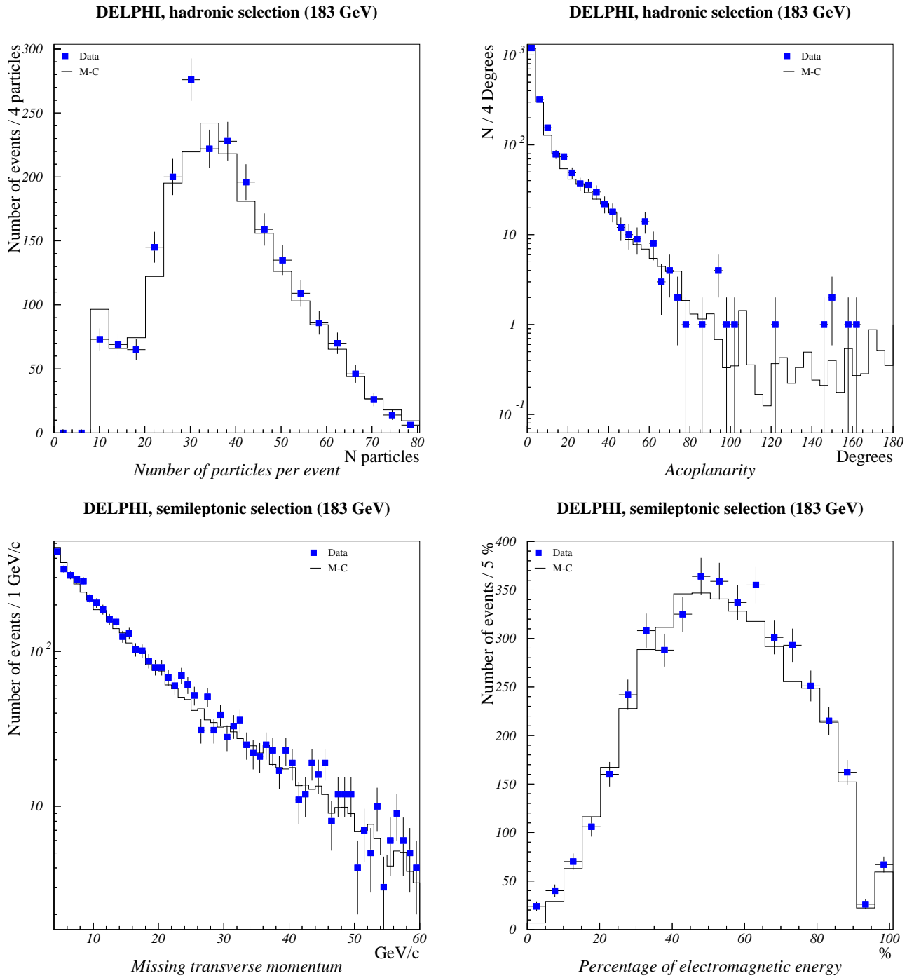
Figure 1: Distributions of total multiplicity and scaled acoplanarity after hadronic topology selection [2]. Distributions of missing transverse momentum and percentage of electromagnetic energy after the semileptonic topology selection [2]. Points show distributions for real data events, histograms for simulated events. The normalization of the histograms is absolute.
