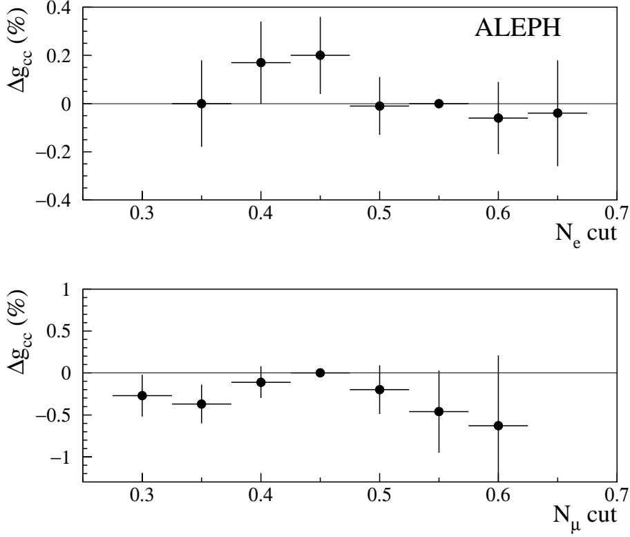
Figure 5: \Delta g_{cc} versus the N_e , N_\mu cut. The error bars indicate the uncorrelated uncertainties.
