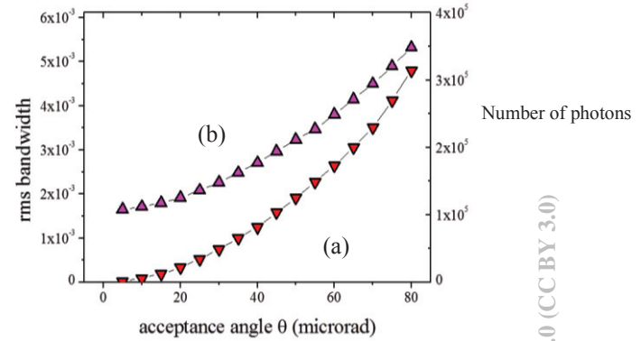
Figure 1: The total number of photons (a) and relative bandwidth (b) vs the rms acceptance angle of the data obtained by adopting the paramtrs reported in Table 2.
