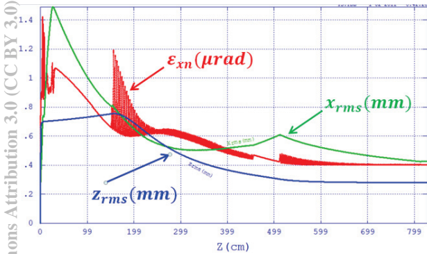
Figure 3: Electron beam emittance, envelope and bunch length evolution in the photoinjector.
