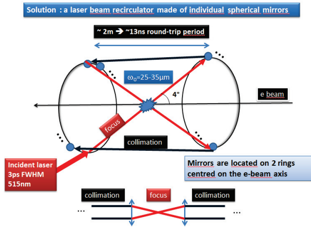
Figure 5: Optical recirculator schematic layout.
