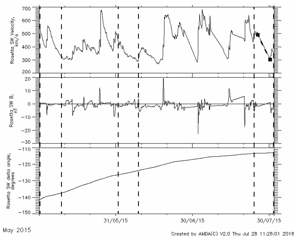
Figure 7. Propagated solar wind parameters using the so-called Tao model [Tao et al. , 2005]. Shown are (top) the radial solar wind velocity, (middle) the tangential magnetic field, and (bottom) the angle between the location of Earth and Rosetta. The dashed vertical lines show the intervals that are discussed in the draping section: 1–8 May, 2–9 June, and 24–31 July. The two black squares in Figure 7 (top) show the location of a data gap in the July interval.
