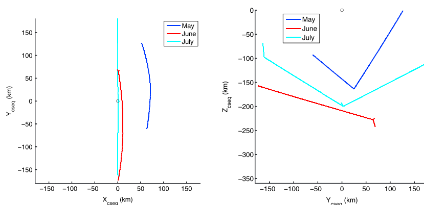
Figure 2. Three partial pyramidal orbits of Rosetta around comet 67P/CG for several days in May, June, and July in the CSEQ (left) XY and (right) YZ plane. The small circle at the origin represents comet 67P/CG.
