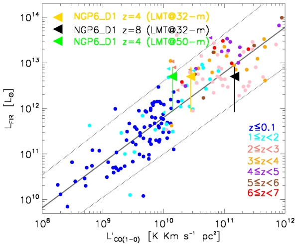
Figure 12. L'_{\text{CO}(1-0)}-L_{\text{FIR}} correlation for (U)LIRGs ( z \leq 0.1 ; Papadopoulos et al. 2012) and DSFGs ( z \geq 1 ; Riechers et al. 2010; Harris et al. 2012; Bothwell et al. 2013; Yun et al. 2015; Aravena et al. 2016; Riechers et al. 2017; Strandet et al. 2017; Yang et al. 2017; Zavala et al. 2018; Gullberg et al. 2018; Jiménez-Andrade et al. 2018) from the literature at different redshifts (coloured circles and legends). Overplotted is the parametrized L'_{\text{CO}(1-0)}-L_{\text{FIR}} relation proposed by Greve et al. (2014; grey solid line) with the associated scatter of the data (grey dotted lines). We show our CO luminosity upper limits for z = 4 and z = 8 solution represented by the yellow and black triangles, respectively, with vertical error bars of the size of FIR luminosity uncertainty obtained in Section 3.2. We also show the same z = 4 solution for a non-detection, but observed with RSR at LMT@50 m (green triangle), which will be near twice the depth of our current RSR observations at LMT@32 m.
