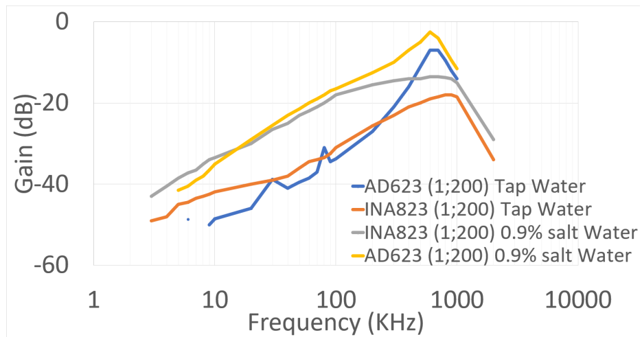
Fig. 9. Rx output signal gain in phantom
