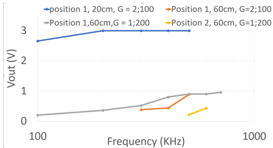
Fig. 13. Output Rx signal amplitude on a Bluefin tuna in different position
