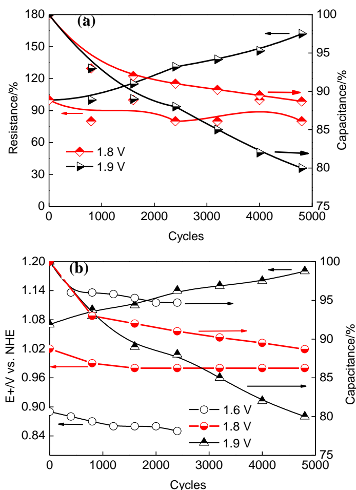
Figure 40 Capacitance retention ratio ( C_n/C_1 \times 100 , where C_n is the capacitance at n^{\text{th}} cycle and C_1 at 1 st cycle) and (a) resistance variation ratio ( R_n/R_1 \times 100 , where R_n is the resistance at n^{\text{th}} cycle and R_1 at 1 st cycle) or (b) maximum potential ( E^+ ) of the positive electrode vs. NHE during galvanostatic ( 200 \text{ mA g}^{-1} ) cycling of a symmetric AC/AC supercapacitor. Electrolyte: 2 \text{ mol L}^{-1} \text{ Li}_2\text{SO}_4 .
