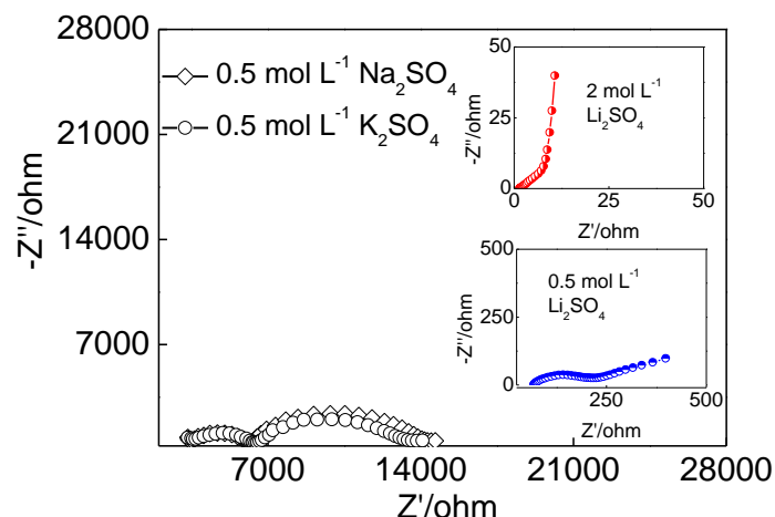
Figure 31 Nyquist plots of symmetric carbon/carbon capacitors in alkali sulfates at -10\text{ }^{\circ}\text{C} .
