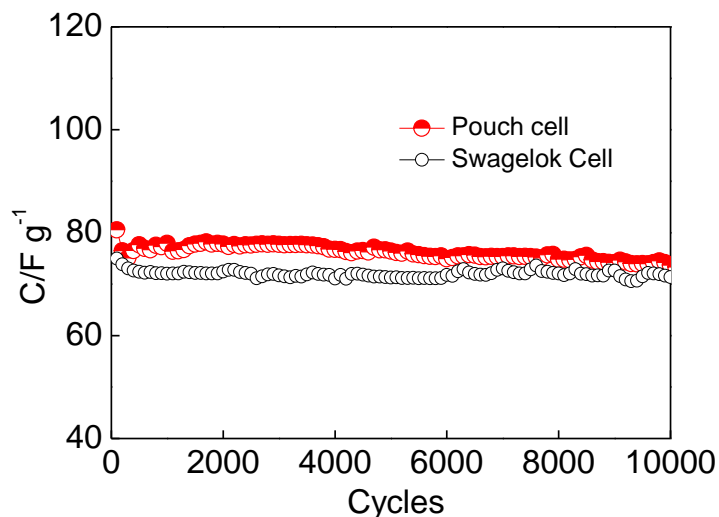
Figure 56 Evolution of discharge capacitance during galvanostatic ( 1 \text{ A g}^{-1} ) cycling of symmetric ACX/ACX Swagelok and pouch cells operating at 2.1 \text{ V} in 2 \text{ mol L}^{-1} \text{ Li}_2\text{SO}_4 electrolyte.
