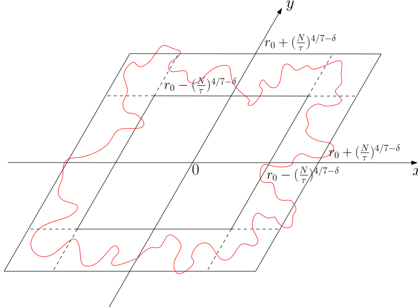
Figure 3.4: Annulus S_{r_0 \pm (\frac{N}{\tau})^{4/7-\delta}} with its divisions and a closed curve.
