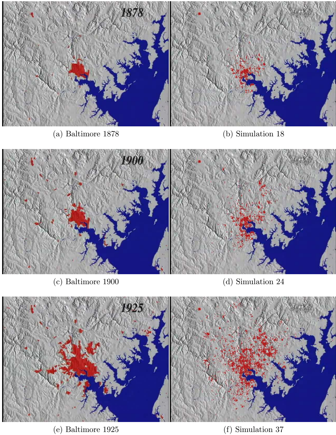
Figure 4.25: Real Baltimore and its simulation (cont)
