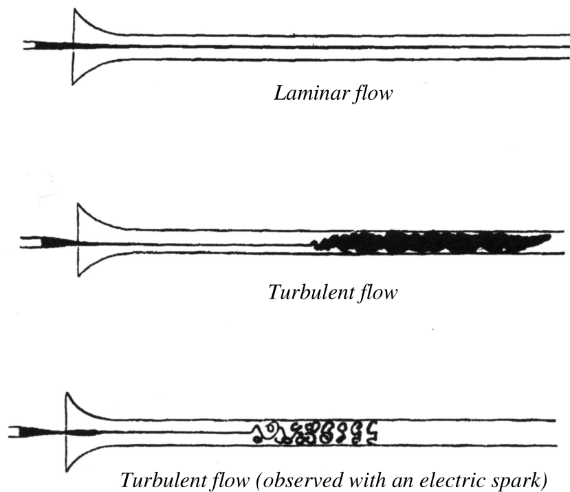
Fig. 2.2.: Sketch of the transition from laminar (top) to turbulent flow (middle) from Reynolds (1883) . The bottom panel shows the same turbulent flow when observed with the light of an electric spark to reveal the "eddies" (now viewed as vortices) of the flow.
