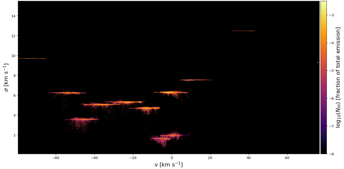
Fig. 4.17.: Two-dimensional probability distribution function \sigma - v weighted by the fraction of total emission of each Gaussian \sqrt{2\pi}a_n\sigma_n/\sum_r N_{HI}(\mathbf{r}) of NEP. The NEP is mainly composed of negative intermediate velocity components.
