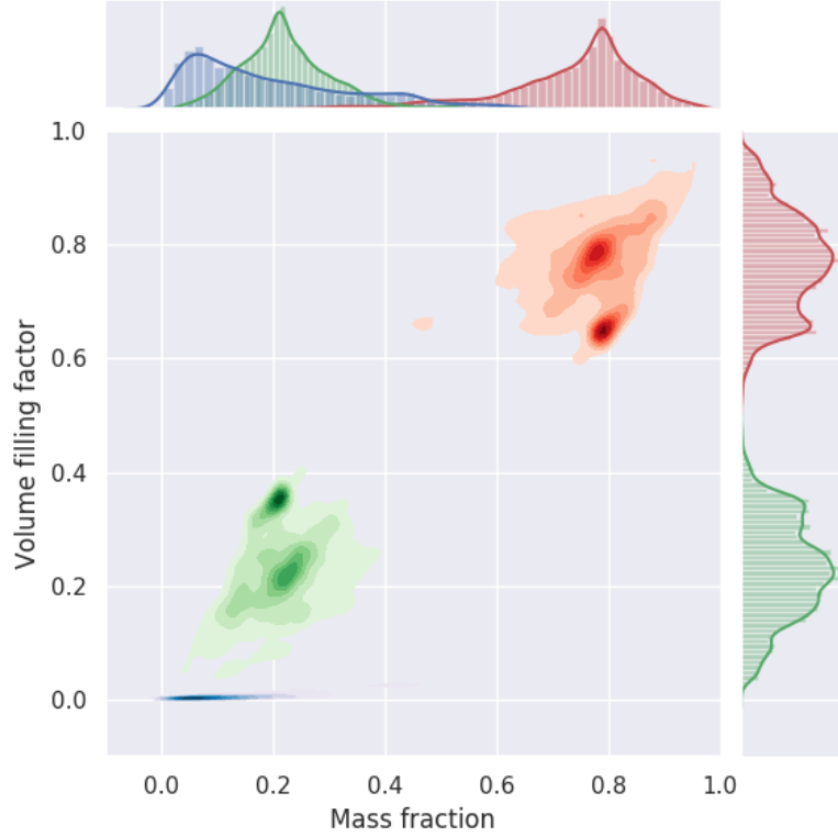
Fig. 5.10.: Two dimensional probability distribution function of the volume filling factor as function of the mass fraction for the WNM (red), LNM (green) and CNM (blue) along each line of sight of a 256 \times 256 \times 1024 pixels region with moderate CNM fraction (same region as in Marchal et al. (2019) of the numerical simulation of thermally bi-stable turbulence performed by Saury et al. (2014) .
