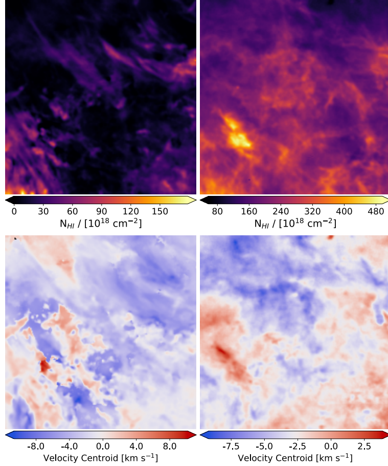
Fig. 4.21.: Left : CNM; Right : inter-cloud medium (WNL+LNM) in NEP inferred with ROHSA. The top and bottom panels show the column density and centroid velocity fields, respectively.
