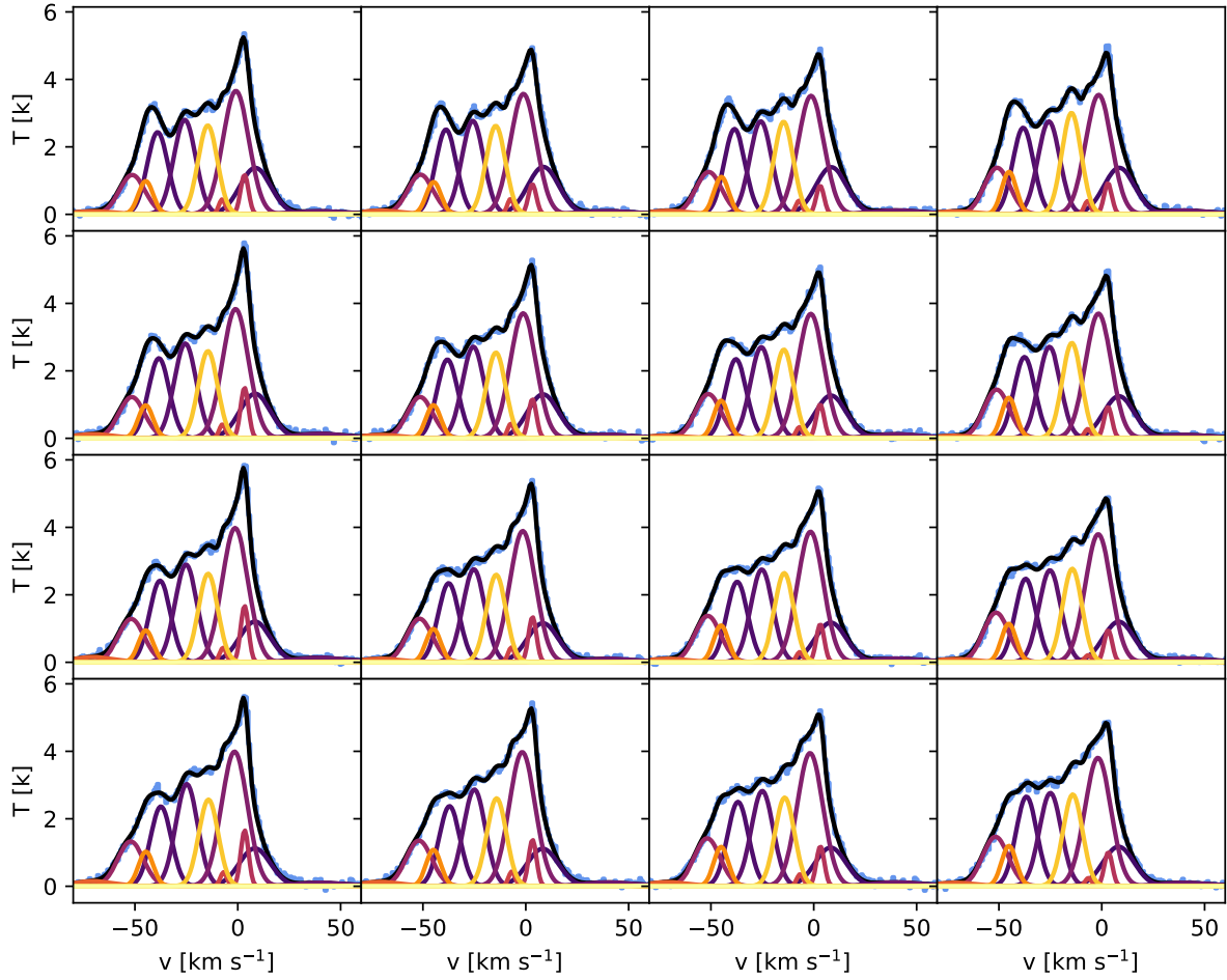
Fig. 4.16.: Example of the Gaussian decomposition obtained by ROHSA (colored line) for a random 4x4 mosaic of NEP. The original signal is shown by the blue histogram and the total brightness temperature encoded by ROHSA is shown in black. The other lines detail the components of the Gaussian model. The spatial coherence of the solution can be seen over the mosaic with a smooth variation of the amplitude, central velocity, and velocity dispersion of each Gaussian component.
