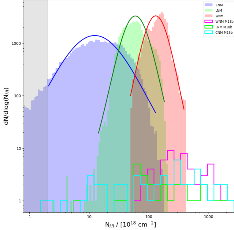
Fig. 5.3.: dN/d\log(N_{HI}) diagram of the CNM (blue), LNM (green) and WNM (red). Solid lines are log-normal fits of the distributions. The grey part shows the values that are not considered to fit the model. Integrated column densities inferred from the 21-Sponge survey (Murray et al., 2018b) are added for the WNM (magenta), the LNM (lime) and the CNM (cyan).
