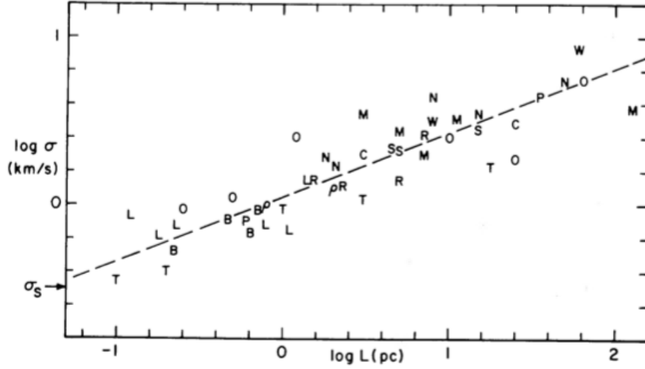
Fig. 2.5.: From Larson (1981) : The three-dimensional internal velocity dispersion \sigma plotted versus the maximum linear dimension L of molecular clouds and condensations, based on data from Table 1; the symbols are identified in Table 1. The dashed line represents equation (1), and \sigma_s is the thermal velocity dispersion.
