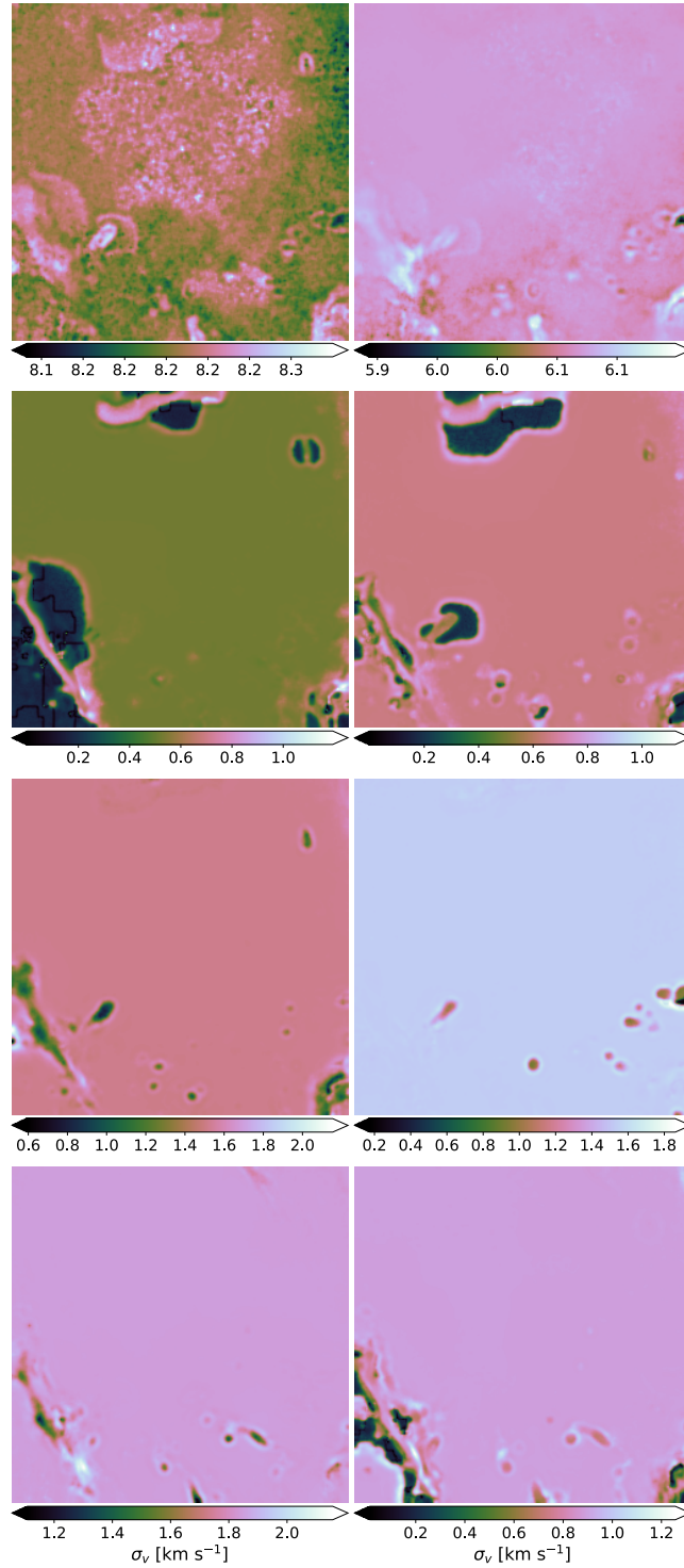
Fig. 4.10.: Dispersion velocity fields \sigma (left : \sigma_1, \sigma_3, \sigma_5, \sigma_7 ; right : \sigma_2, \sigma_4, \sigma_6, \sigma_8 ) obtained by ROHSA using the synthetic observation computed in Sect. 4.2.2.
