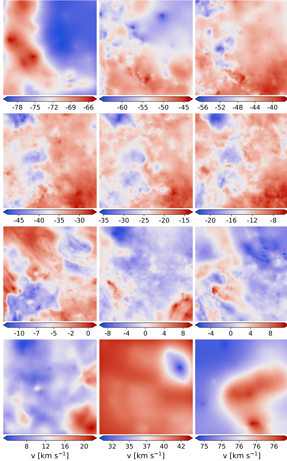
Fig. 4.19.: Centroid velocity fields \mu (left: \mu_1, \mu_4, \mu_7, \mu_{10} ; middle: \mu_2, \mu_5, \mu_8, \mu_{11} ; right: \mu_3, \mu_6, \mu_9, \mu_{12} ) obtained by ROHSA applied on NEP.
