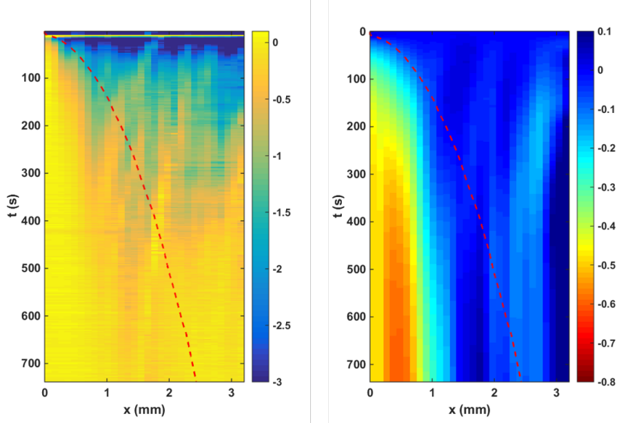
Figure 6.6: Left: spatio-temporal map of the velocity field v_x in the cell, for R_M = 882 . The \text{CaCl}_2 reservoir is on the left, at x = 0 . The velocity field is deduced from individual tracer trajectories, averaged in the transverse direction. The dashed line represents the front evolution, deduced from the grayscale intensity images. Right: from the velocity the total deformation \epsilon is computed as \epsilon = \int_0^t \partial_x v_x .
