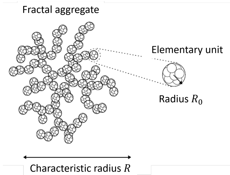
Figure 1.5: Schematic representation of a fractal aggregate of characteristic radius R , made of elementary units of radius R_0 . Figure taken from Aymard et al. (1997), [10]
