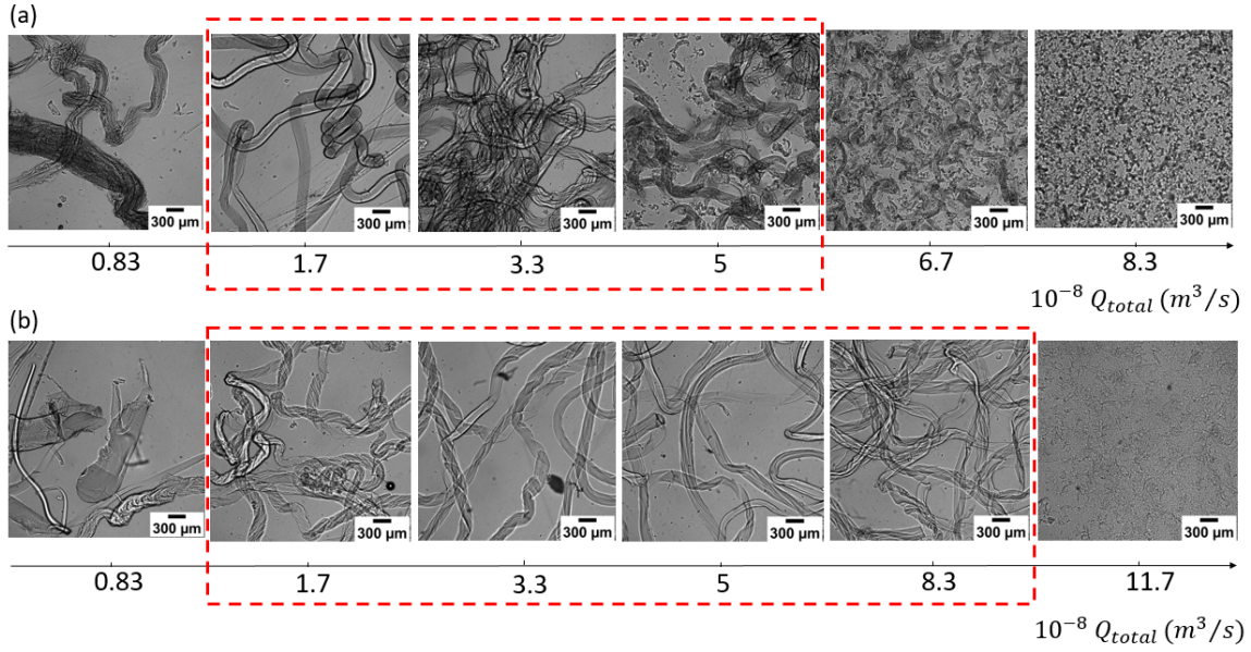
Figure 5.4: Effect of the total flow rate Q_{total} on fiber formation for a fixed residence time ( t_{\text{global}} = 6 \text{ s} ). Fibers were collected in the \text{CaCl}_2 solution used for their fabrication. [\text{WPI}] was fixed at 8% w/w. (a) Molar ratio R_m = 17 and [\text{CaCl}_2] = 68 \text{ mM} . (b) R_m = 335 and [\text{CaCl}_2] = 1.5 \text{ M} . Fibers were obtained for a range of Q_{total} that is outlined by the red dotted boxes.
