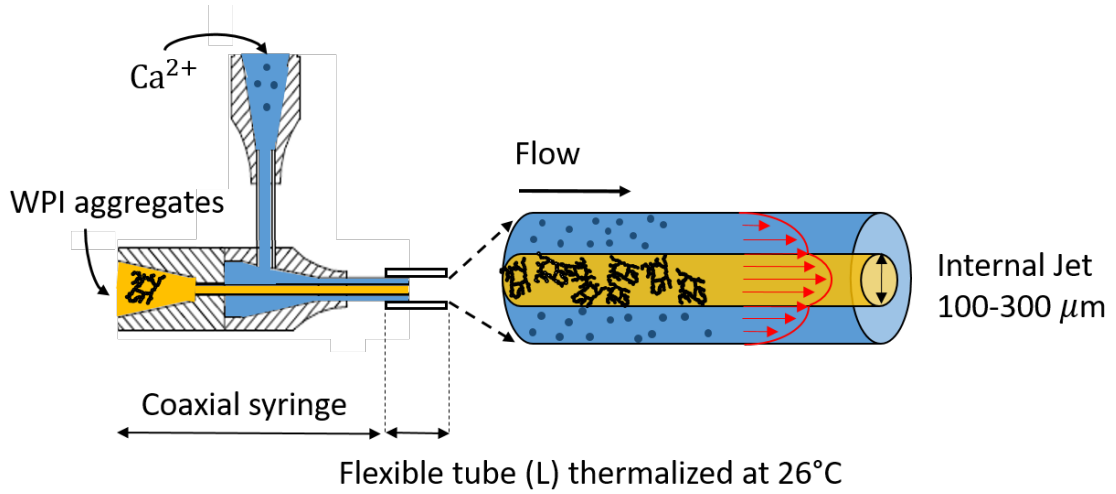
Figure 5.3: Schematic of the co-axial flow focusing device used to produce WPI aggregates fibers by \text{Ca}^{2+} -induced gelation. The co-axial needle was connected to a tube. The tube was immersed in a bath at constant temperature ( 26^\circ\text{C} ). The fibers were collected in a petri dish. The suspension of WPI aggregates was injected via the inner needle (yellow), whereas the solution of calcium was injected by the outer needle (blue).
