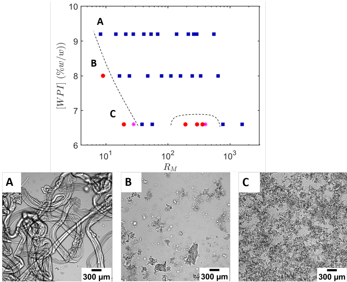
Figure 5.6: State diagram of fibres formation as a function of [WPI] and R_M , after 30 s of their production. Fibres were stored in the calcium solution used for their production. Blue squares: fibers (image A). Red circles: no fibers / microscopic aggregates (images B and C). Pink stars: conditions of transition where both aggregates and short fibers were produced. Dotted lines are a guide for the eyes. Q_{\text{total}} = 3.3 \times 10^{-8} \text{ m}^3/\text{s} , Q_{\text{CaCl}_2}/Q_{\text{agg}} = 10 , t_{\text{global}} = 6 \text{ s} .
