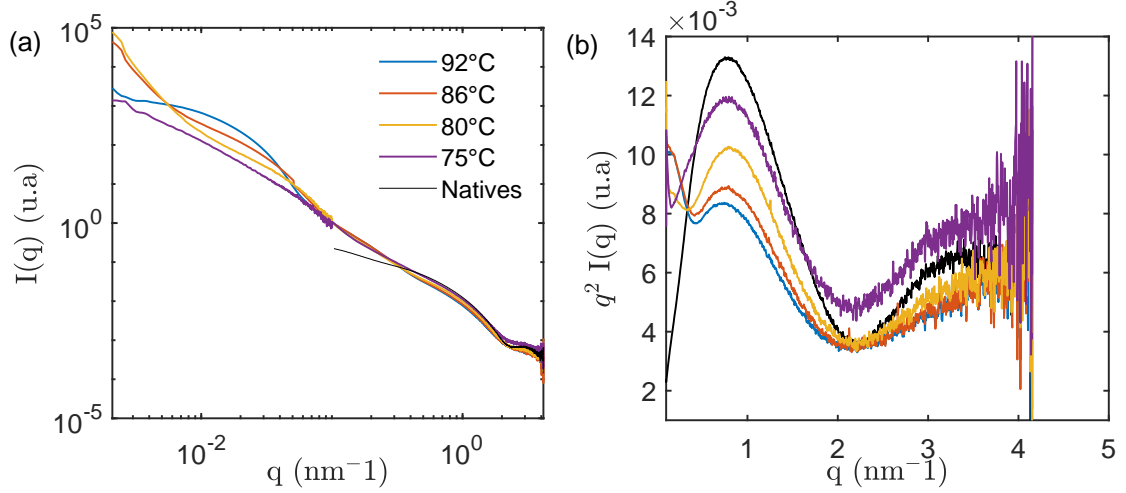
Figure 3.7: a: SAXS intensities I(q) of the WPI aggregates formed at 4% w/w 10 mM pH 7.0 after heat treatment at different temperature of aggregation and t = 300 s. b: Kratky plot showing the evolution of WP conformation for the different temperature of aggregation investigated for t = 300 s, \dot{\gamma} = 53 \text{ s}^{-1} , d = 0.81 \text{ mm} , L = 246 \text{ cm} , Q = 15 \text{ mL/h} .
