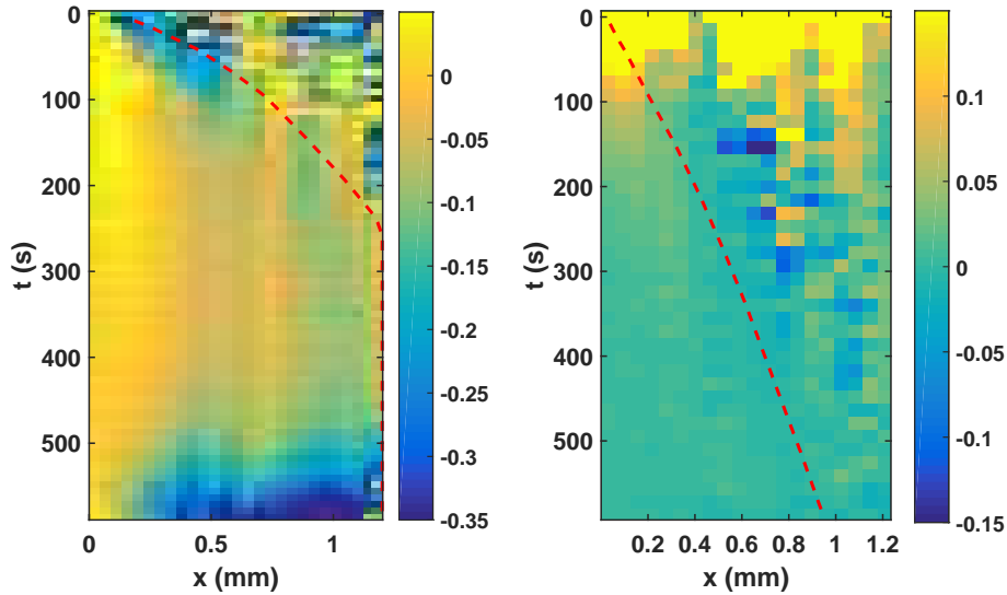
Figure 6.7: Spatio temporal plot of the velocity field in the cell, for R_M = 160 (Left), and R_M = 16 (Right). The dashed line represent the front displacement, obtained from the grayscale images.
