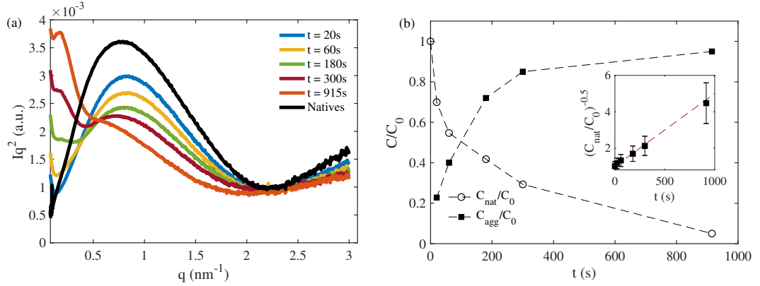
Figure 3.5: a : Kratky plots showing the change of WP conformation with the residence time t . b : the fraction of native WP, C_{\text{nat}}/C_0 was determined from high q -range of spectra ( \circ , Eq. 3.10, 3.11) and was calculated from a linear combination of the spectra of natives and aggregated WPI in the q -range 1-2 \text{nm}^{-1} (dashed lines), see text for details. The fraction of aggregated WP, C_{\text{agg}}/C_0 , was determined independently from the low q -range of spectra ( \blacksquare , Eq. 3.12). Dashed lines are guide for the eyes. In insert, kinetic plot (C_{\text{nat}}/C_0)^{1-n} versus t with reaction order n=1.5 . \dot{\gamma} = 53 \text{ s}^{-1} , d = 0.81 \text{ mm} , Q = 15 \text{ mL/h} , L = 10 - 87 \text{ cm}
