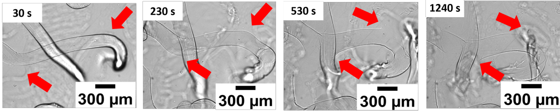
Figure 5.10: Kinetics of swelling and breakage of the fiber at intermediate molar ratio R_M (regime II) during the storage step in \text{CaCl}_2 solutions. a: [\text{WPI}] = 8\% w/w and R_M = 47 . The fibers swelled up to disappear. b: [\text{WPI}] = 9.2\% w/w and R_M = 41 . The shell of the fiber broke-up locally, as shown by red arrows. Q_{\text{total}} = 3.3 \times 10^{-8} \text{ m}^3/\text{s} , Q_{\text{CaCl}_2}/Q_{\text{agg}} = 10 , t_{\text{global}} = 6 \text{ s} .
