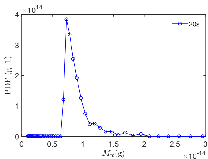
Figure 2.10: Mass-weighted probability density of aggregates. Solution of aggregated proteins at 4% 10 mM NaCl pH7.0 under flow for 20 s at 92°C under an average shear of 32 s -1 .
