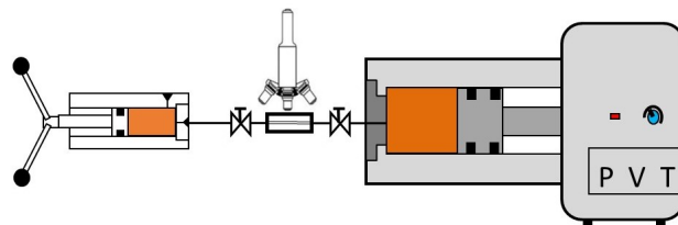
FIGURE 6.19: Schematic of the high pressure microscope set-up
