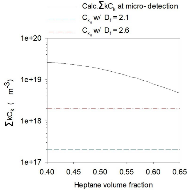
FIGURE 4.14: Calculated cumulative number of primary clusters across all the aggregates at the time of microscope detection
