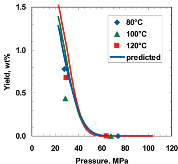
FIGURE 6.10: Reported by Tharanivasan et al. 40 : Modeled yield of unstable asphaltenes from a depressurized live-oil
