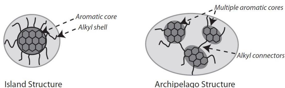
FIGURE 1.3: Schematic of the island and archipelago structures of asphaltene molecules (reproduced from Hoepfner 28 )
