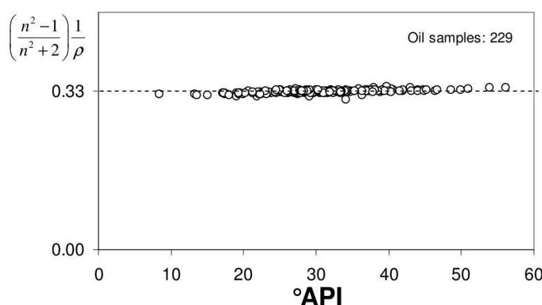
FIGURE 1.18: Consistency of the one-third rule applied to more than 200 stabilized crude oils at atmospheric pressure (reprinted from Vargas and Chapman 70 )
