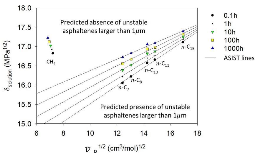
FIGURE 6.32: Predictions of ASIST solubility lines to experimental instability of asphaltene obtained by constant mass expansion of methane-oil and measured by microscopy for several aging times and several n -alkanes versus the square-root of the partial molar volume of the used n -alkane ( v_p^{1/2} )
