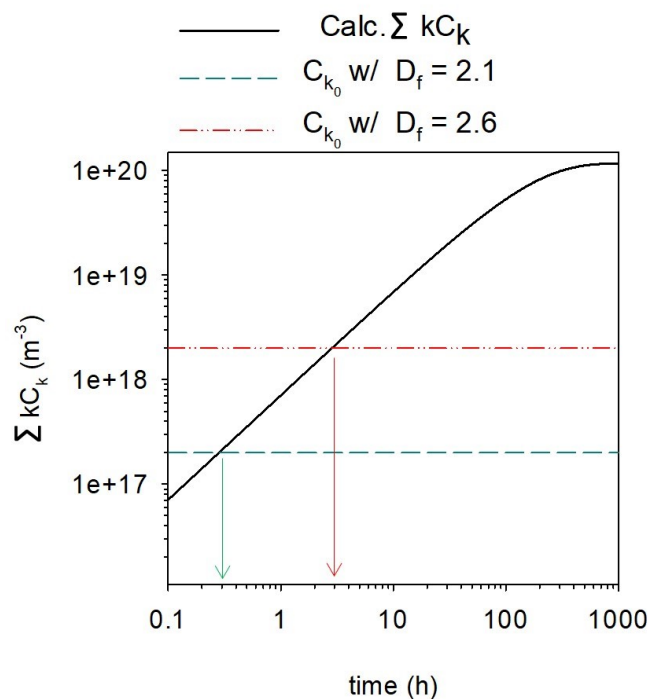
FIGURE 4.7: Comparison between the total number of primary particles across all entities and the minimum concentration of particles C_{k_0} to enable microscope observations for the case of heptane content = 47 vol%
