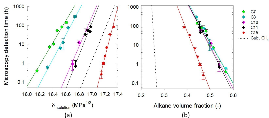
FIGURE 6.28: Calculated microscopy detection-time curve of unstable asphaltenes induced by methane (along with other n -alkanes previously showed) as a function of (a) the solubility parameter of oil-alkane solutions and (b) the volume fraction of respective alkanes
