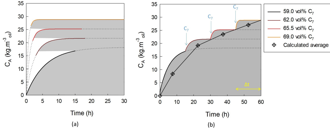
FIGURE 3.17: Comparison of the modeled evolution of the total concentration of unstable asphaltenes C_A as a function of time for: (a) independent solutions prepared at time = 0 (b) a tracked solution with series of step additions of heptane
