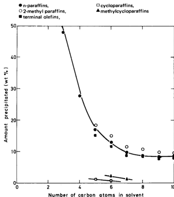
FIGURE 6.3: Reported by Mitchell and Speight 26 : Relation of amount of precipitated asphaltenes to the number of carbon atoms in non-aromatic solvents
