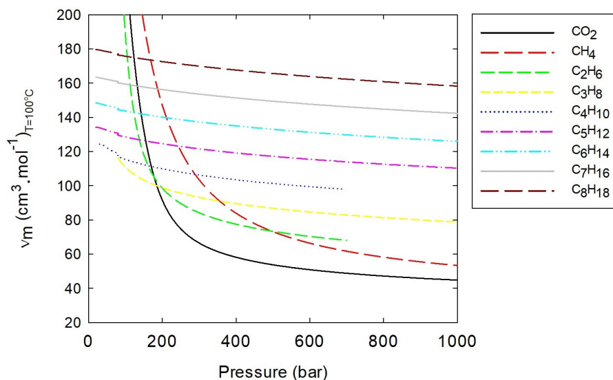
FIGURE 1.20: Pure molar volumes of the 9 lightest main components of live-oils as a function of the hydrostatic pressure in typical range of oil & gas industrial pressures at 100 °C(reprinted from NIST chemical web book)
