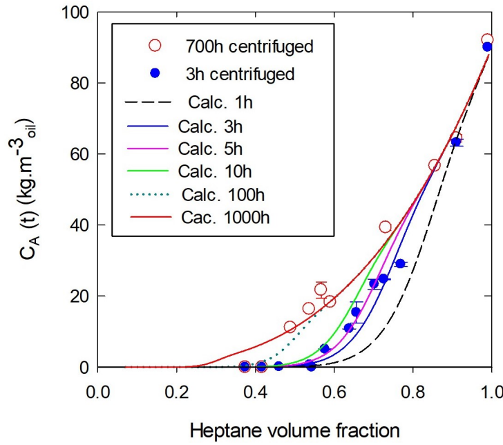
FIGURE 3.15: Concentration of unstable asphaltenes C_A versus the heptane content for solutions aged for different times
