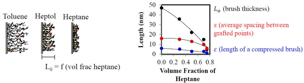
FIGURE 4.2: Measured repulsive interactions between asphaltenes particles using an AFM and interpreted length of steric brushes 28;27
