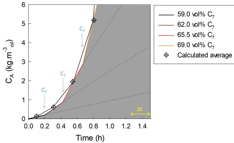
FIGURE 3.18: Modeled evolution of the total concentration of unstable asphaltenes C_A as a function of time during the continuous addition of heptane at a flow rate q_{C_7} = 0.3 \text{ cm}^3.\text{min}^{-1}
