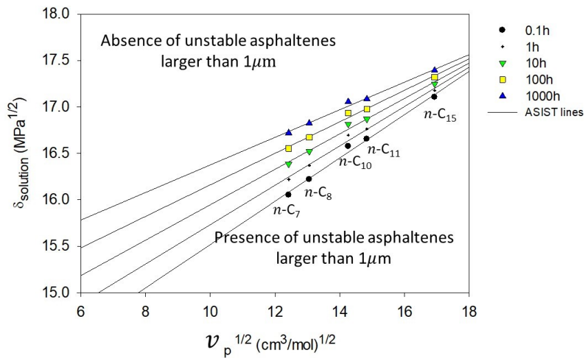
FIGURE 6.22: Solubility parameter of solutions corresponding to the microscope detection of unstable asphaltenes for several aging times and several n -alkanes versus the square-root of the partial molar volume of the used n -alkane ( v_p^{1/2} )
