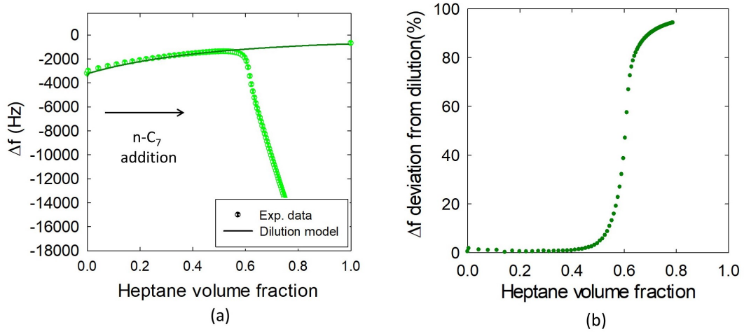
FIGURE 2.10: (a) Comparison between experimental and dilution correlated (eq.2.9) frequency shifts versus heptane volume fraction for the 3 rd overtone at 60°C (b) Percent deviation of the measured data from the calculated dilution curve.
