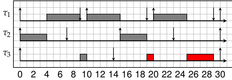
Figure 1.5.: The DM task scheduling (unschedulable case)
