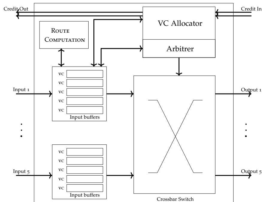
Figure 2.6.: Router architecture
