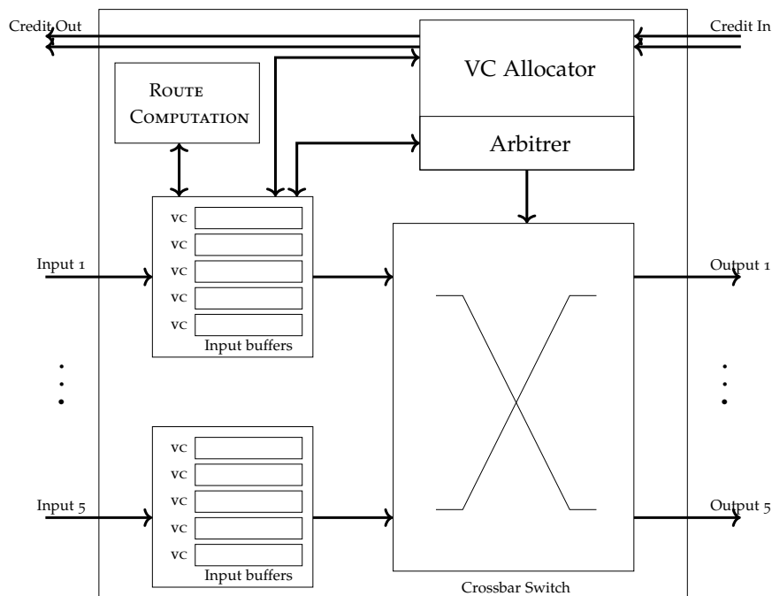
Figure 2.6.: Router architecture
