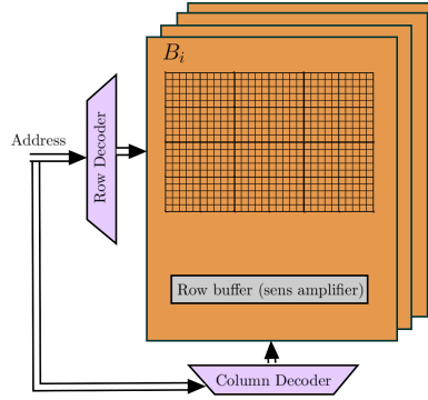
Figure 6.2.: DRAM architecture
