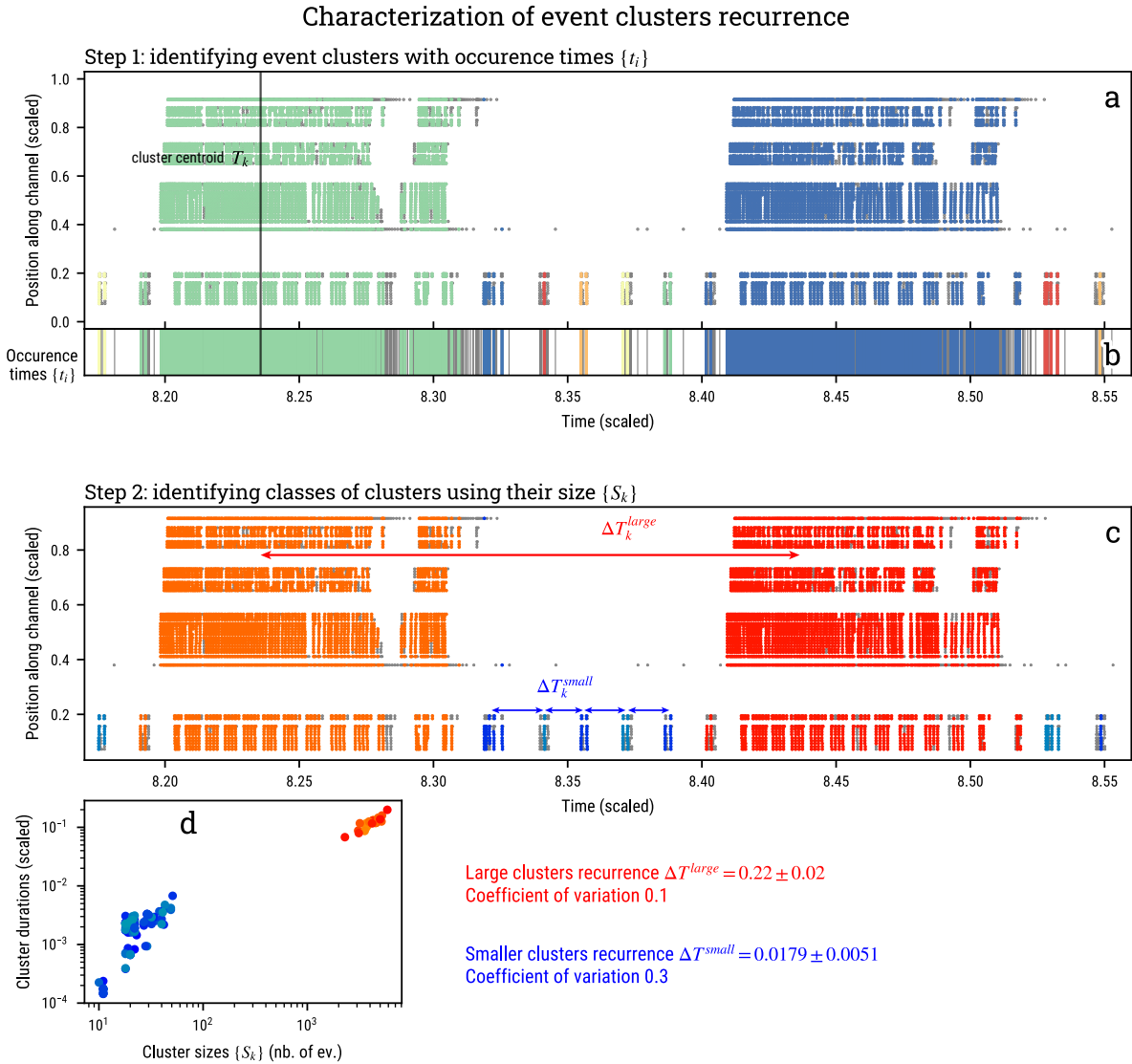
Figure 4.3 — Recurrence analysis of a simulated, highly clustered activity in a clustered valve system with N_v = 43 valves ( \bar{d}_v = 1w_v ), u = 0.3 , under a input flux of q_{in} = 0.16 (activity count in Figure 4.2a). In a first step, the algorithm detects clusters of events using the occurrence times. (a) Time-dip representation of activity, each point corresponds to an events. Events are colored according to which cluster they are labelled into. The grey dots are labelled as noise, either in the de-noising step, or by the clustering algorithm. The clustering algorithm is performed only on occurrence times, represented as horizontal lines in (b), with the same color-coding as in (a). The centroid of each cluster T_k is computed as the average occurrence time of events that belong to each one of them. In a second step, clusters of events are grouped into classes, based on their sizes. Two sizes of clusters are detected for this simulation, small clusters in blue shades, and large clusters in orange to red shades. (c) Time-dip representation of events, with events colored according to the cluster and class they belong to. The delays \Delta T_k between cluster centroids of each class are indicated with arrows. (d) The size-duration distribution of clusters of events. The classifying step only considers the size of clusters.
