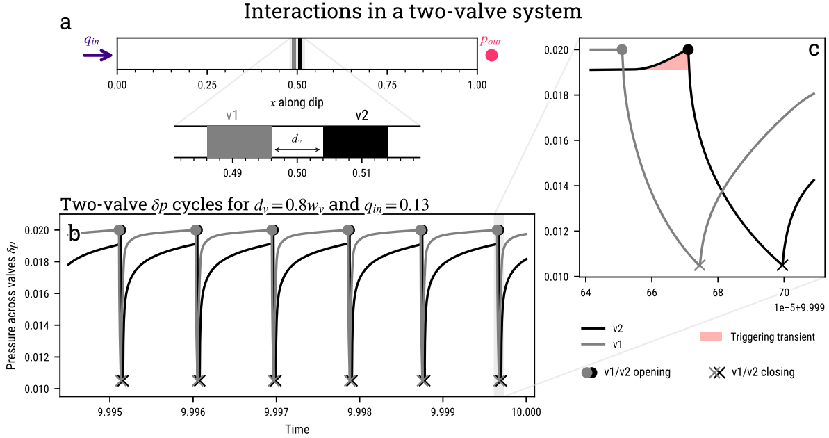
Figure 4.4 — Interactions in a two-valve system. (a) A system with two valves ( v1 and v2 ) spaced by d_v = 0.008 = 0.8w_v , submitted to a constant flux q_{in} = 0.13 , and a constant pressure output p_{out} = 0 . (b) Cycles of fluid pressure accumulation and release pressure are shown with the time-series of the pressure difference \delta p across v1 and v2 . Closing and opening events are indicated, and occur when \delta p reaches a pre-defined threshold. (c) As v1 opens first and when v2 is critically stressed, the pressure transient its opening produces (in red) triggers the opening of v2 , with a short delay.
