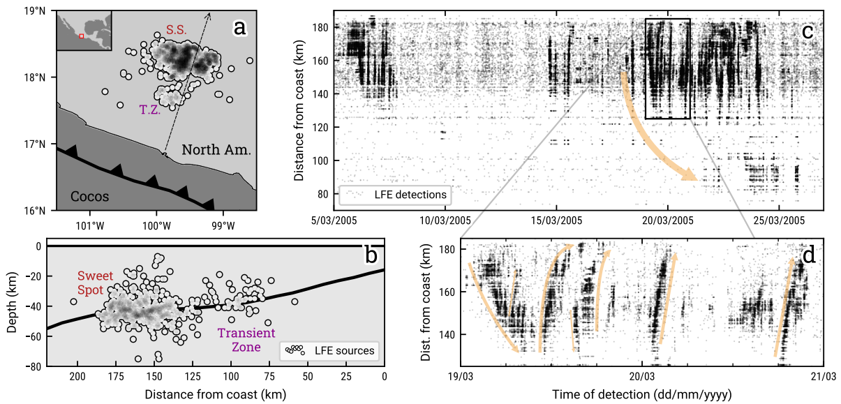
Figure 3.1 — The Guerrero (Mexico) tremor zone in (a) map view and (b) vertical cross-section. Each dot represents a low-frequency earthquake family from Frank et al. (2014). Thick black lines outline the trench and the subduction interface (data from Hayes (2018)). (c) and (d), LFE activity in a time-location chart from the Frank et al. (2014) catalog. Activity occurs in two patches centered on the subduction interface, a dense downdip one called the sweet spot and a sparser updip one called the transient zone. Tremor activity migrates along the subduction interface in both the updip and downdip directions, as shown by the orange arrows.
