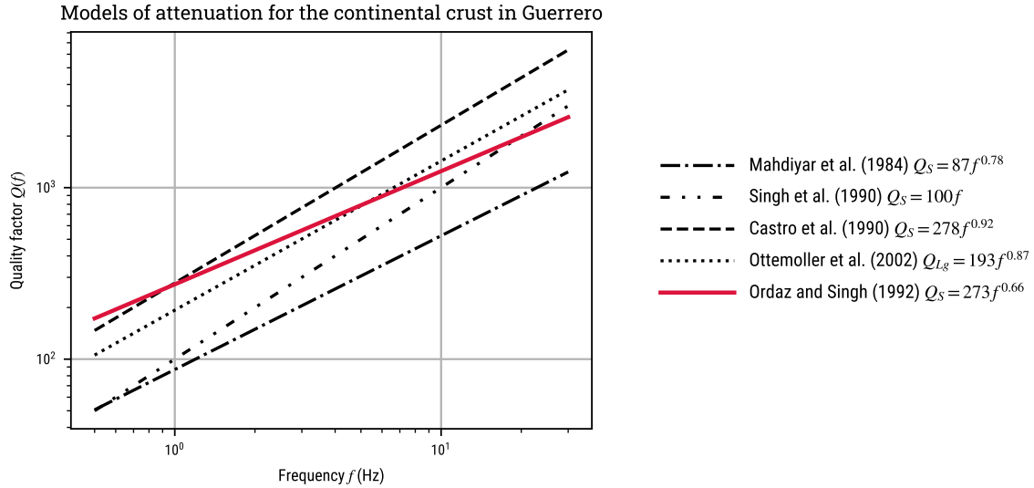
Figure 2.B.1 — Models of attenuation for the crust of Guerrero. All modeled frequency-dependent quality factors are measured on the S-waves of regional earthquakes, which wave travel through the crust of Guerrero, except for the model by Ottemöller et al. (2002), who measured it on the Lg phase.
