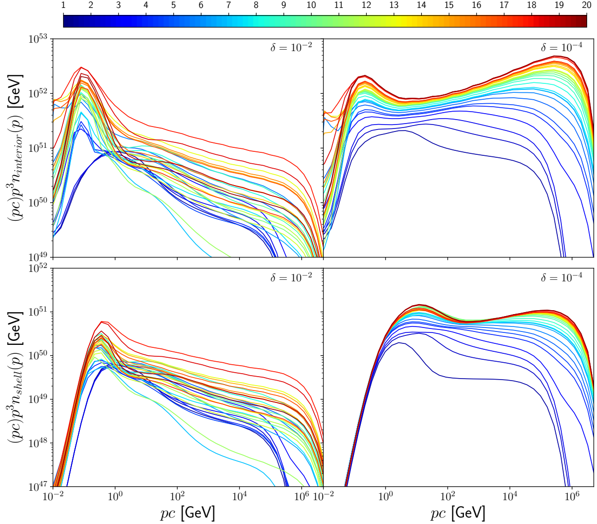
Figure 6.10: Average spectra in a two-zone (top panels: interiors, bottom panels: shells) model with two different values of the shell confinement coefficient \rho_b/\delta = 10 (left panels), 1000 (right panels). Each curve corresponds to a different time represented by the colour scale in units of Myr at the top.
