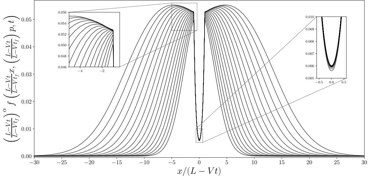
Figure 4.5: Spatial distribution of accelerated particles in rescaled coordinates (see text). Curves refer to different times between Vt_i/L = 0.9 and Vt_f/L = 0.98 , and for a momentum at t_i equal to p/p_i = 10 . The best match between solutions at different times is found for values of \alpha gradually approaching \sim 4 as we increase the resolution of the numerical scheme.
