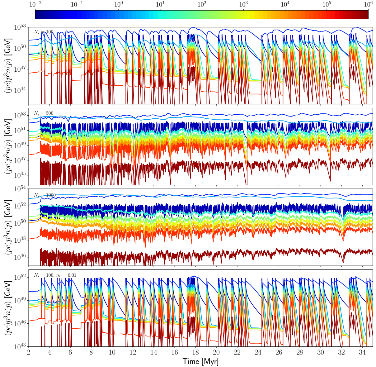
Figure 6.5: Time evolution of the particle distribution function. The parameters of the superbubble are highlighted in red in Table 6.1. Top panel: 100 massive stars. Second panel: 500 massive stars. Third panel: 1000 massive stars. Bottom panel: 100 massive stars, with \eta_T = 1\% instead of 30%. Colours correspond to different momenta (see the colour scale in units of GeV/c at the top). Dark blue: 10 MeV/c. Blue: 0.13 GeV/c. Light blue: 1.6 GeV/c. Turquoise blue: 20 GeV/c. Green: 240 GeV/c. Yellow: 2.9 TeV/c. Orange: 35 TeV/c. Red: 0.43 PeV/c. Dark red: 5.3 PeV/c.
