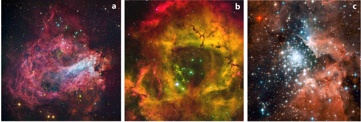
Figure 1.8: Interstellar bubbles. (a) Composite image of the Omega nebula (M17). (b) The Rosette nebula in false colours (SII in blue, [OIII] in green, H\alpha in red). (c) NGC3603 in three optical wavelengths: 435 nm (blue), 550 nm (green), 850 nm (red).
