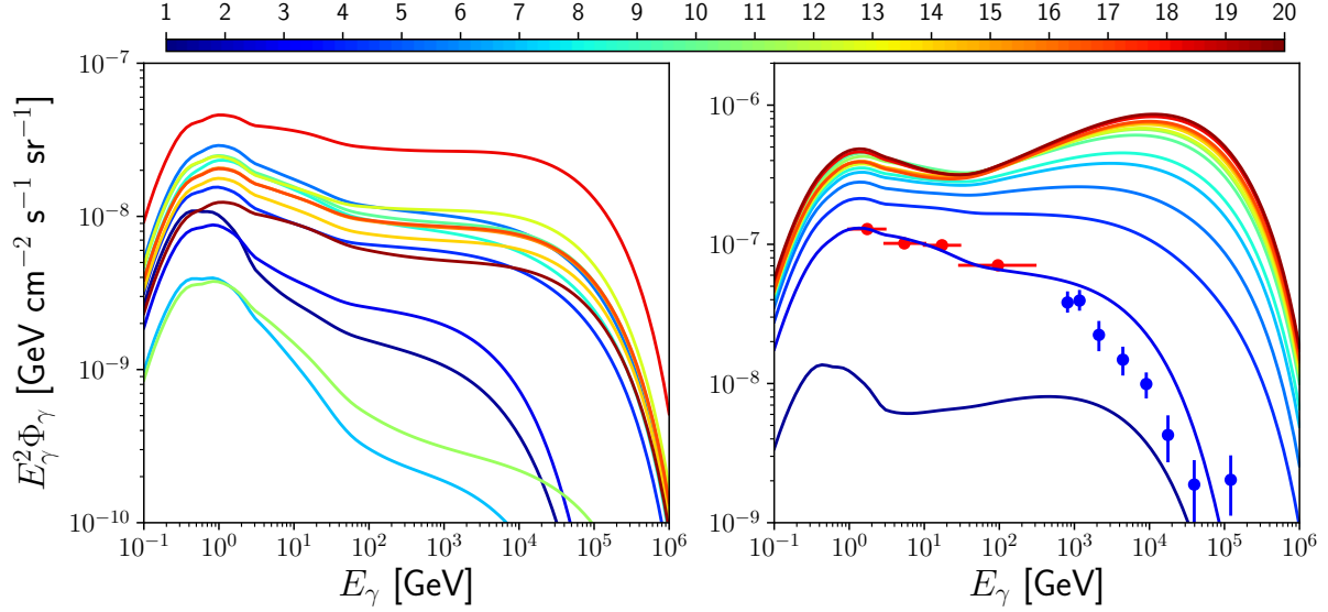
Figure 6.12: Gamma-ray spectral energy distributions from p-p interactions in a standard superbubble shell of hydrogen number density n_H = 30 \text{ cm}^{-3} ( n_{ISM} = 10 \text{ cm}^{-3} ), with a shell confinement coefficient \rho_b/\delta = 10 (left panel), and 1000 (right panel). The source is a loose cluster of 100 massive stars located at 1.5 kpc from the Earth. Spectra are plotted at various times from 1 to 20 Myr corresponding to the various colours from blue to red (see the colour scale at the top). The data points show the gamma-ray flux measured in the Cygnus region: Fermi-LAT data in red (Abdollahi et al., 2020) and HAWC data in blue (Abeysekara et al., 2021).
