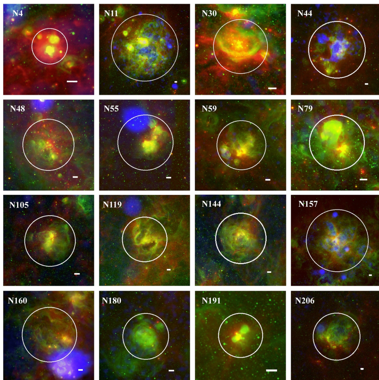
Figure 1.11: Multi-wavelength observations of superbubbles in the Large Magellanic Cloud (red: 24\ \mu\text{m} , green: \text{H}\alpha , blue: X-rays). The white bar has a length of 1' ( \sim 14.5\ \text{pc} ). Figure adopted from Lopez et al. (2014).
