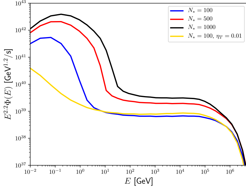
Figure 6.7: Average flux of cosmic rays escaping the superbubble.
