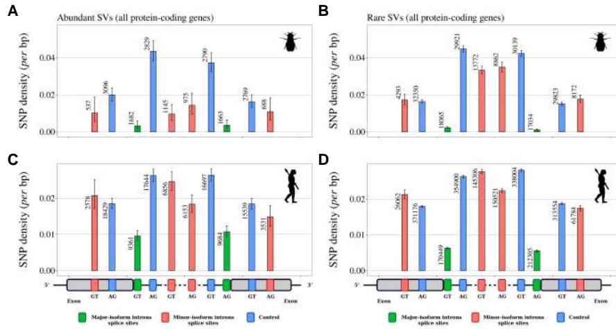
Figure 6.5: Variation in selective constraints on alternative splice signals from rare and abundant SVs. For each minor-isofom intron sharing one boundary with a major-isofom intron, we measured the SNP density at its minor splice site (red), and at the corresponding major splice site (green). We distinguished minor splice sites that are located in an exon or in an intron of the major isofom. As a control (blue), we selected AG or GT dinucleotides that are unlikely to correspond to alternative splice sites, namely: AG dinucleotides located toward the end of the upstream exon or the beginning of the intron (unlikely to correspond to a genuine acceptor site), and GT dinucleotides located toward the beginning of the downstream exon or the end of the intron (unlikely to correspond to a donor site). To increase the sample size, we analyzed data from all annotated protein-coding genes (and not only the BUSCO gene set). The number of sites studied is shown at the top of each bar. Error bars represent the 95% confidence interval of the proportion of polymorphic sites (proportion test). A,B: SNP density in Drosophila melanogaster (polymorphism data from 205 inbred lines derived from natural populations, N=3,963,397 SNPs (Huang et al., 2014; Mackay et al., 2012)). C,D: SNP density in Homo sapiens (polymorphism data from 2,504 individuals, N=80,868,061 SNPs (Auton et al., 2015)). We excluded dinucleotides affected by CpG hypermutability (Materials & Methods, see Appendix Fig. A.6 for CpG sites). A,C: Abundant SVs (MIRA > 5%). B,D: Rare SVs (MIRA \leq 5%).
